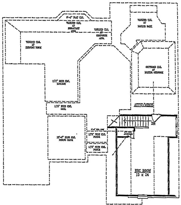
SECOND LEVEL FLOOR PLAN
