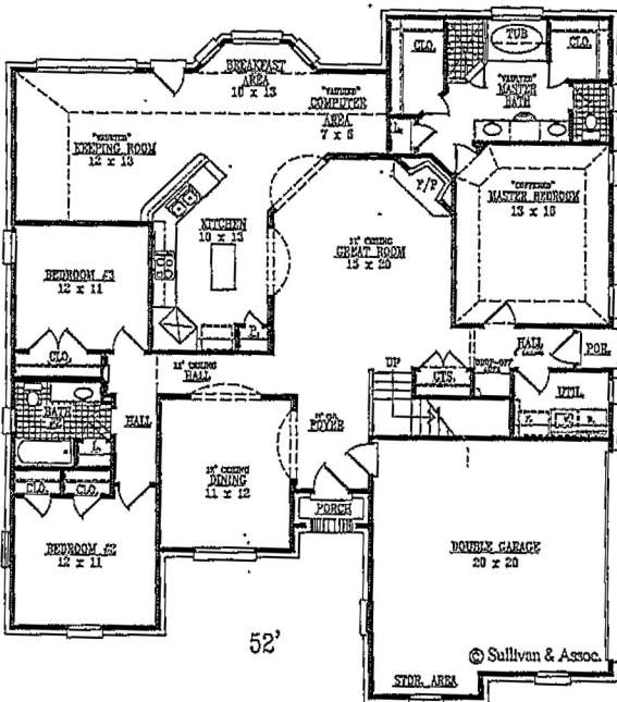
FIRST LEVEL FLOOR PLAN
